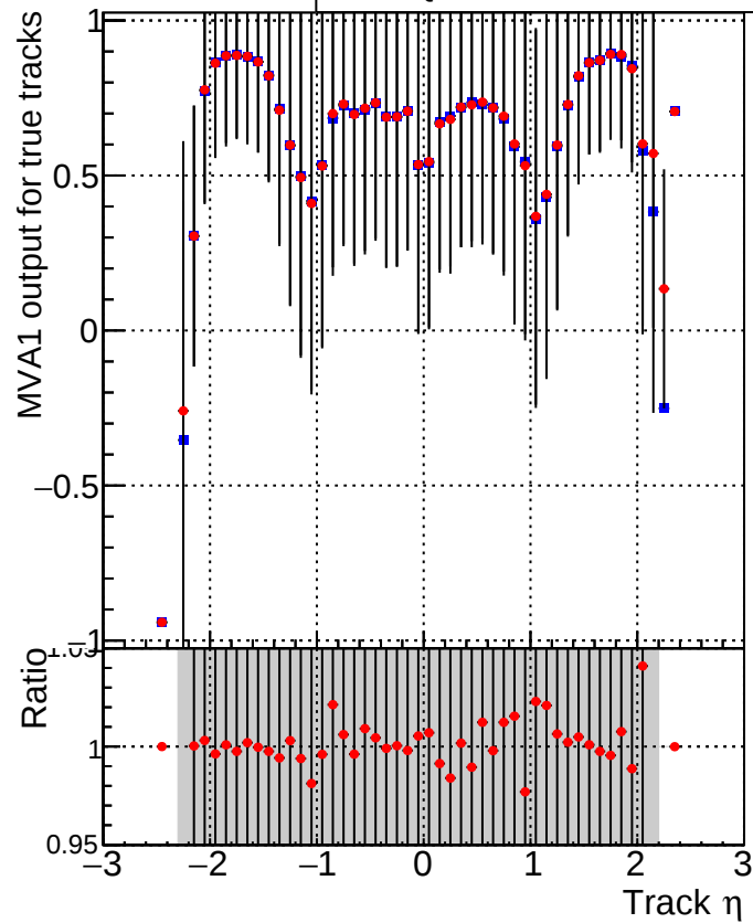
MVA1 of associated tracks (recoToSim) vs. track \eta Legend: ■ DQM_mkFit_TToriginal ● DQM_mkFit_TTNEWSH_ALLITERS
