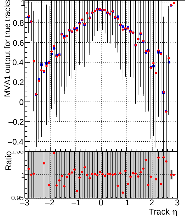
MVA1 of associated tracks (recoToSim) vs. track \eta Legend: ■ DQM_mkFit_TToriginal ■ DQM_mkFit_TTNEWSH_ALLITERS
