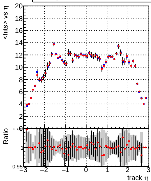
mean hit — DQM_mkFit_TToriginal — DQM_mkFit_TTNEUHS_ALLITERS
