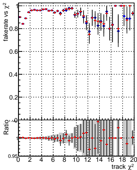
Fake rate vs. —●— DQM_mkFit_TToriginal —●— DQM_mkFit_TTNEWSH_ALLITERS
