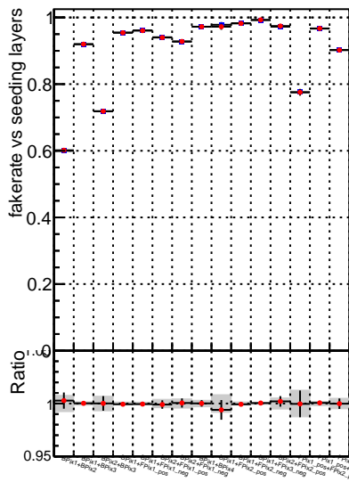
Fake rate vs. —●— DQM_mkFit_TToriginal —●— DQM_mkFit_TTNEWSH_ALLITERS
