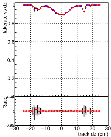
—•— DQM_mkFit_TToriginal —•— DQM_mkFit_TTNEWHS_ALLITERS
