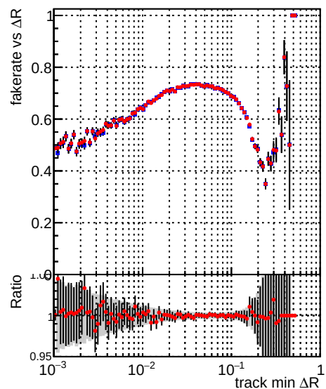
Fake rate vs \Delta R (track, jet) Legend: —•— DQM_mkFit_TToriginal —•— DQM_mkFit_TTNEWHS_ALLITERS
