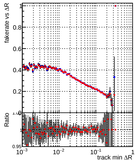
—•— DQM_mkFit_TToriginal —•— DQM_mkFit_TTNEWHS_ALLITERS
