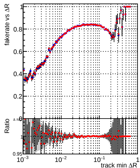
Fake rate vs DQM_mkFit_TToriginal DQM_mkFit_TTNEWS ALLITERS
