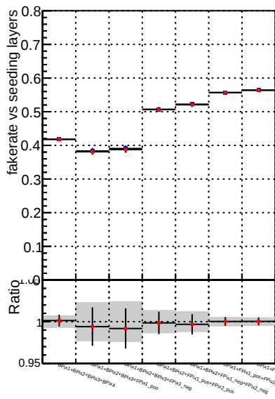
Fake rate vs. —•— DQM_mkFit_TToriginal —•— DQM_mkFit_TTNEWS ALLITERS
