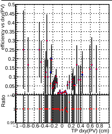
Efficiency vs Dxy(PV) DQM_mkFit_TToriginal DQM_mkFit_TTNEWSH_ALLITERS
