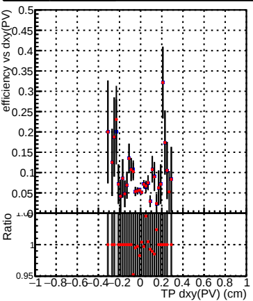
Efficiency vs Dxy(PV) Legend: DQM_mkFit_TToriginal (black line with blue markers), DQM_mkFit_TTNEWHS_ALLITERS (red line with markers)
