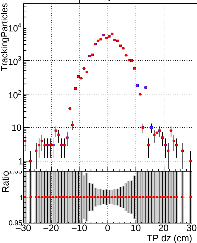
■ DQM_mkFit_TToriginal ● DQM_mkFit_TTNEWHWS_ALLITERS
