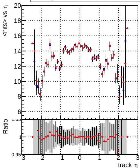
— DQM_mkFit_TToriginal — DQM_mkFit_TTNEWHS_ALLITERS
