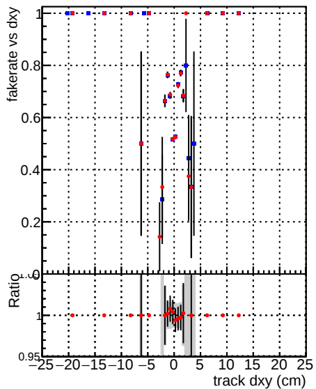
—■— DQM_mkFit_TToriginal —●— DQM_mkFit_TTNEWSH_ALLITERS
