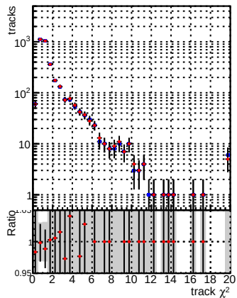
N of reco track vs. \chi^2 —●— DQM mkFit TToriginal —●— DQM mkFit TTNEWHS_ALLITERS
