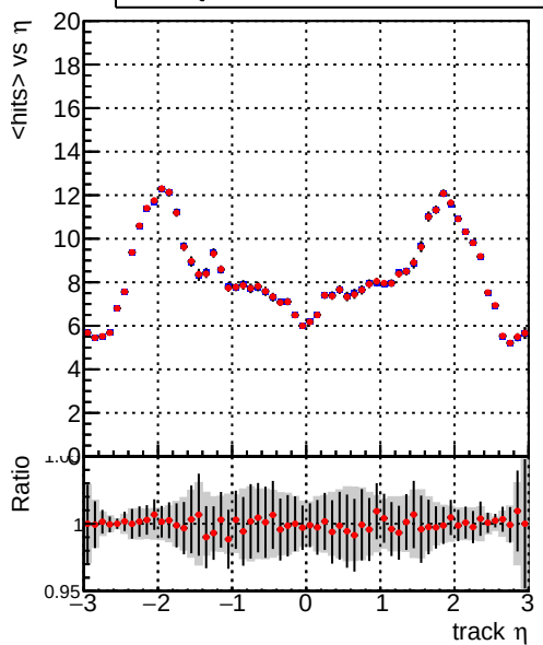
mean hit — DQM_mkFit_TToriginal — DQM_mkFit_TTNEUHS_ALLITERS
