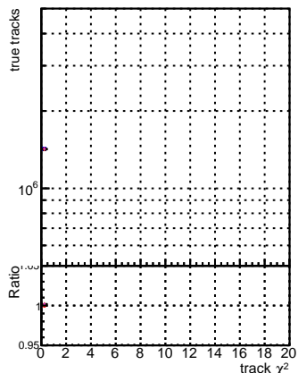
N of reco track vs. \chi^2 for original vs. ALLITERS-106, NEWHS-3700, ALLITERS-196
