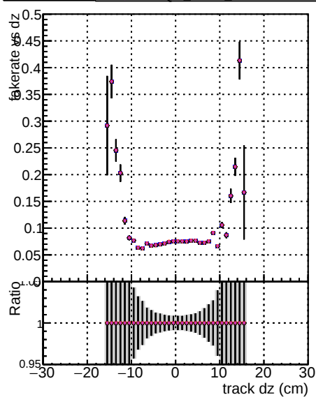
Legend for Fake rate vs d, Duplicates Rate vs Dxy, and Pileup rate vs dxy plots: DOM mkrFit T-Original-106 DOM mkrFit T-NEWHSM3100-ALLITERS-106 DOM mkrFit T-NEWHSM3100-ALLITERS-106
