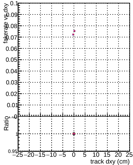
Legend for Fake rate vs d, Duplicates Rate vs Dxy, and Pileup rate vs dxy plots: DOM mkrFit T-Original-106 DOM mkrFit T-NEWHSM3100-ALLITERS-106 DOM mkrFit T-NEWHSM3100-ALLITERS-106
