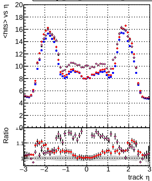
mean hit DOM mkFit TToriginal-106 DOM mkFit TTNEWHSMS ALLITERS-106 DOM mkFit TTNEWHSMS50 ALLITERS-106 DOM mkFit TTNEWHSMS100 ALLITERS-106
