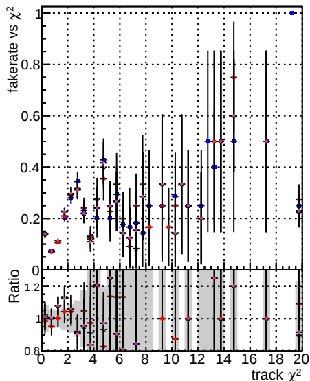
Fake rate vs. \chi^2 for ALLTIPS 106 and NEWHSM3500 ALLTIPS 106
