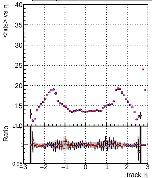
mean hits vs \eta DOM mkFit Toriginal-106 DOM mkFit TNEWSMS ALLITERS-106 DOM mkFit TNEWSMS50 ALLITERS-106 DOM mkFit TNEWSMS100 ALLITERS-106
