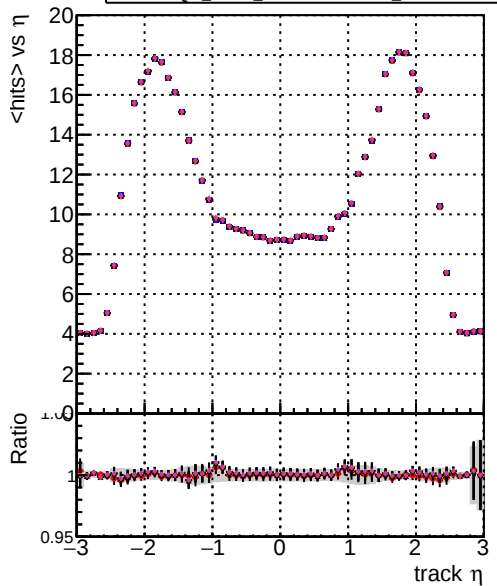
Legend: DOM mkFit TToriginal-106, DOM mkFit TTNEWSMS ALLITERS-106, DOM mkFit TTNEWSMS50 ALLITERS-106, DOM mkFit TTNEWSMS100 ALLITERS-106 mean hits vs \eta
