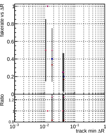
Fake rate vs \Delta R(\text{track, jet}) DQM mkFit Toriginal T106 T350 T500 TNEW TSM TALL TERS-106 TERS-350 TERS-500 TERS-NEW TERS-SM TERS-ALL
