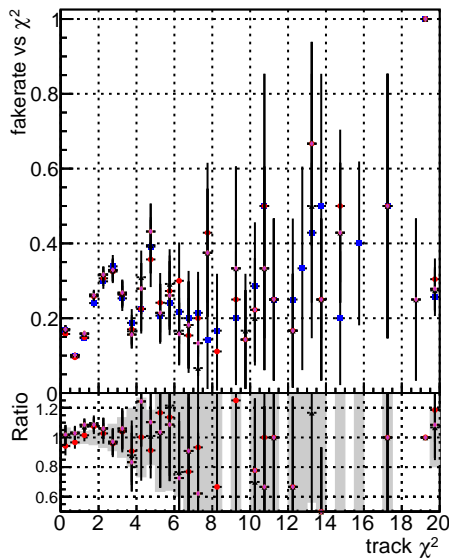
Fake rate vs. DQM mkFit Toriginal Tnew Tnew390 Tnew106 Tnew196
