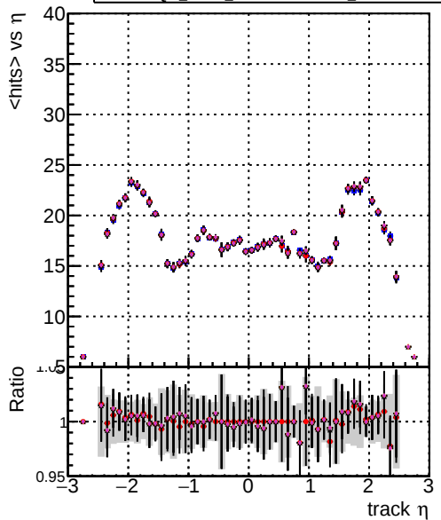
mean hits DOM mkFit Toriginal-106 DOM mkFit TNEWSMS ALLITERS-106 DOM mkFit TNEWSMS50 ALLITERS-106 DOM mkFit TNEWSMS100 ALLITERS-106
