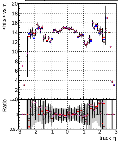
mean hits vs \eta DOM mkFit Toriginal-106 DOM mkFit TNEWHSM50 ALLITERS-106 DOM mkFit TNEWHSM50 ALLITERS-106 DOM mkFit TNEWHSM100 ALLITERS-106
