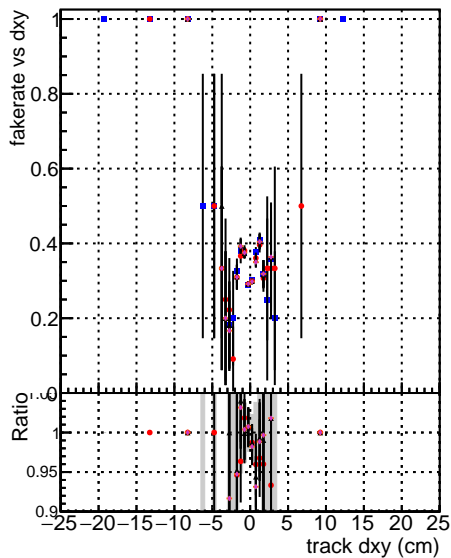
Legend for Fake rate vs dxy: DQM mkrFit Toriginal Toriginal vs ALLITERS-106 NEW HSM3700 ALLITERS-106 ALLITERS-106
