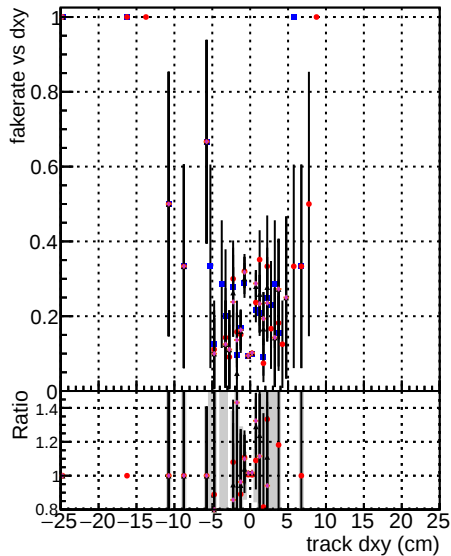
Legend for Fake rate vs dxy, Duplicates Rate vs Dxy, and Pileup rate vs dxy: DOM mkr fit DOM mkr fit + Toriginal DOM mkr fit + Toriginal + Tnew DOM mkr fit + Toriginal + Tnew + TSM DOM mkr fit + Toriginal + Tnew + TSM + TALLTIPS DOM mkr fit + Toriginal + Tnew + TSM + TALLTIPS + T106 DOM mkr fit + Toriginal + Tnew + TSM + TALLTIPS + T106 + T109 DOM mkr fit + Toriginal + Tnew + TSM + TALLTIPS + T106 + T109 + T106
