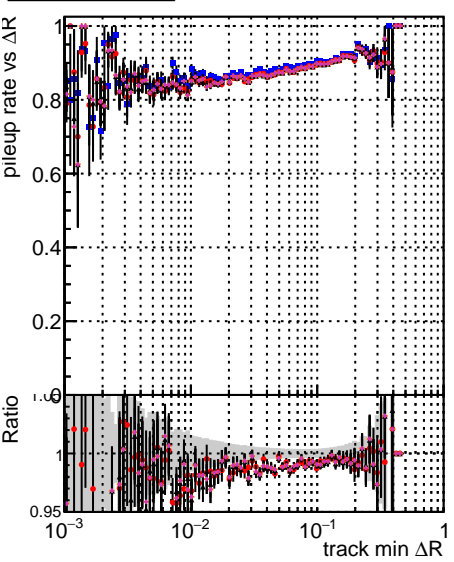
Fake rate vs \Delta R(\text{track}, \text{jet}) | Duplicates rate vs \Delta R(\text{track}, \text{jet}) | Pileup rate vs \Delta R(\text{track}, \text{jet}) Legend: DOM, MKFIT, ORIGINAL, ALLITERS-106, DQM, MKFIT, NEW, HSM, S500, ALLITERS-106
