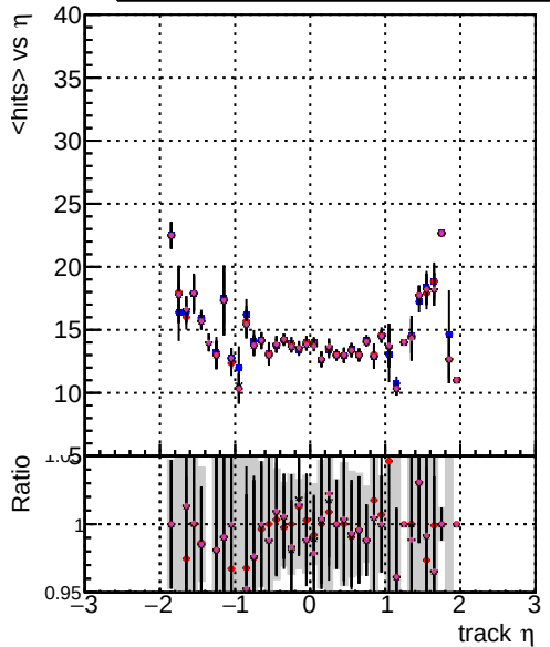
mean hits DOM mkFit Toriginal-106 DOM mkFit TNEWHSMS ALLITERS-106 DOM mkFit TNEWHSMS50 ALLITERS-106 DOM mkFit TNEWHSMS100 ALLITERS-106
