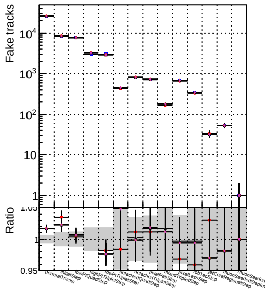
DOM mkFit TTOriginal-106 DOM mkFit TTOriginal-106 ALLITERS-106 DOM mkFit TTNEWSMS50 ALLITERS-106 DOM mkFit TTNEWSMS100 ALLITERS-106
