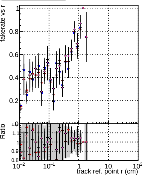
Fake rate vs v Legend: BQM, mkFit, Toriginal, Tfit, NEWHSMS, ALLITERS-106, NEWHSMS-106, ALLITERS-106
