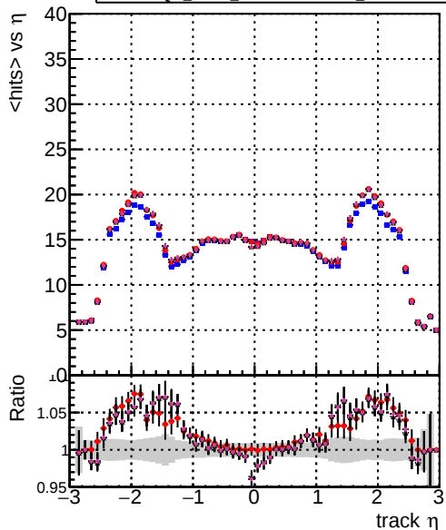
mean hit DOM mkFit Toriginal-106 DOM mkFit TNEWHSM50 ALLITERS-106 DOM mkFit TNEWHSM100 ALLITERS-106
