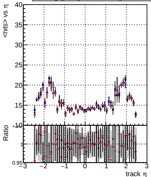
Legend for mean hits vs \eta : DOM mkFit Toriginal-106 DOM mkFit TNEWSMS ALLITERS-106 DOM mkFit TNEWSMS50 ALLITERS-106 DOM mkFit TNEWSMS100 ALLITERS-106
