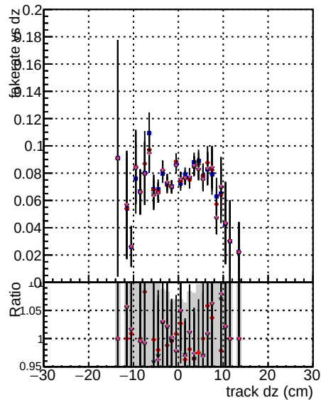
Fake rate vs dz DOM mkr fit T original 106 ALLITERS 106 DOM mkr fit T NEWISM3500 ALLITERS 106
