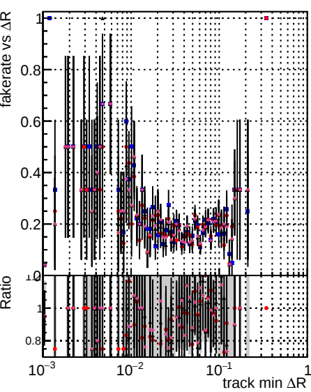
Fake rate vs \Delta R(\text{track, jet}) Legend: DOM (blue circles) mkFit (red circles) Toriginal (black circles) NEWHSM35106 (green circles) ALLITERS106 (purple circles)
