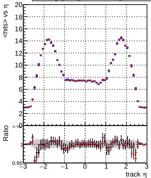
DOM mkFit Toriginal-106 DOM mkFit TNEWHSMS ALLITERS-106 DOM mkFit TNEWHSMS50 ALLITERS-106 DOM mkFit TNEWHSMS100 ALLITERS-106 mean hits
