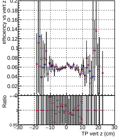
Efficiency vs. TP vert z Legend: - DOM mkFit TToriginal-106 - DOM mkFit TTNEWSMS ALLITERS-106 - DOM mkFit TTNEWSMS50 ALLITERS-106 - DOM mkFit TTNEWSMS100 ALLITERS-106
