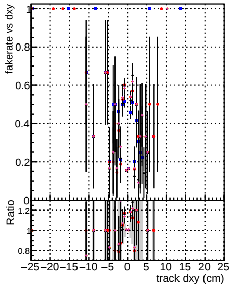
Legend for Fake rate vs dxy, Duplicates Rate vs Dxy, and Pileup rate vs dxy: DOM mkr fit TT original fit ALL TERS 106 DOM mkr fit TT original fit ALL TERS 106 DOM mkr fit TT original fit ALL TERS 106
