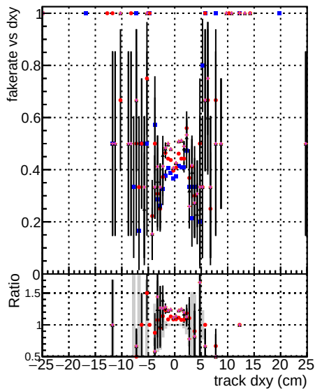
Legend for Fake rate vs dxy: DOM mkr fit T original vs ALLITERS 106 DOM mkr fit T NEW HSM 3500 ALLITERS 106 DOM mkr fit T NEW HSM 3500 ALLITERS 106
