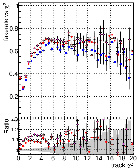
Fake rate vs. DOM mkFit T Original vs ALLTIPS 106 DOM mkFit T NEWISM3100 ALLTIPS 106
