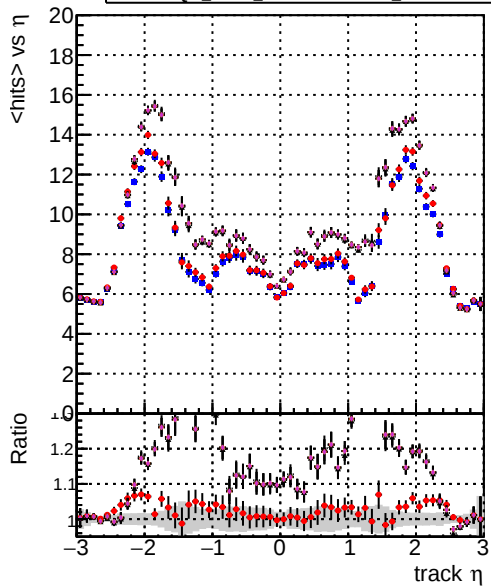
mean hits vs \eta DOM mkFit Toriginal-106 DOM mkFit TNEWHSMS ALLITERS-106 DOM mkFit TNEWHSMS50 ALLITERS-106 DOM mkFit TNEWHSMS100 ALLITERS-106
