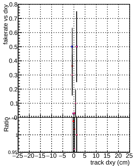
DOM mktFit Toriginal 106 ALLITERS 106 DOM mktFit TNEW 3500 ALLITERS 106
