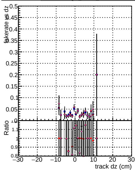
DOM mktFit Toriginal 106 ALLITERS 106 DOM mktFit TNEW 3500 ALLITERS 106
