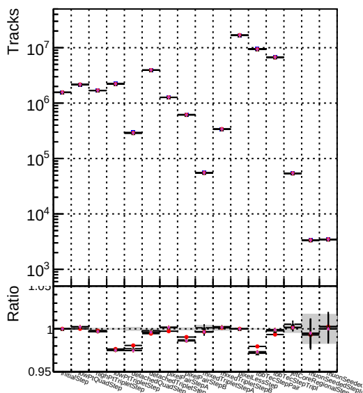
Number of tracks vs collection Legend: DOM mkFit Toriginal-106 DOM mkFit TNEWHSMS95 ALLITERS-106 DOM mkFit TNEWHSMS50 ALLITERS-106 DOM mkFit TNEWHSMS100 ALLITERS-106
