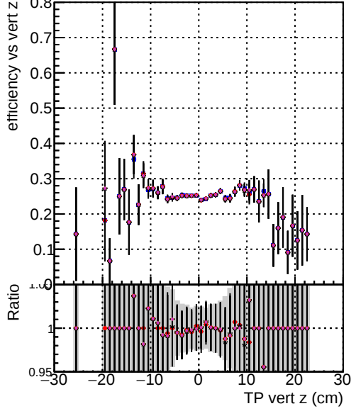
Efficiency vs. TP vert z (cm) DOM mkFit TToriginal-106 DOM mkFit TTNEWHSMS95 ALLITERS-106 DOM mkFit TTNEWHSMS50 ALLITERS-106 DOM mkFit TTNEWHSMS100 ALLITERS-106
