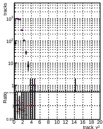
N of reco track vs. \chi^2 for DOM mFit TITAN Original vs. DOM mFit TITAN NEWFSM300 ALLTIPS-106
