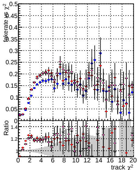
Fake rate vs. DOM mkFit T original pos ALLITERS-106 DOM mkFit T NEW HSM3100 ALLITERS-106
