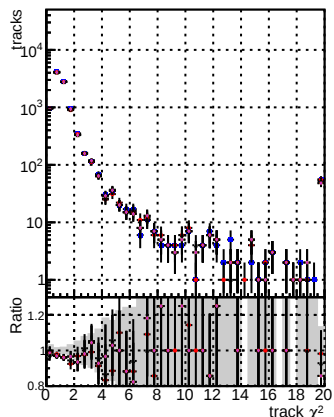
N of reco track vs. \chi^2 for BOM, M1, M2, M3, M4, M5, M6, M7, M8, M9, M10, M11, M12, M13, M14, M15, M16, M17, M18, M19, M20, M21, M22, M23, M24, M25, M26, M27, M28, M29, M30, M31, M32, M33, M34, M35, M36, M37, M38, M39, M40, M41, M42, M43, M44, M45, M46, M47, M48, M49, M50, M51, M52, M53, M54, M55, M56, M57, M58, M59, M60, M61, M62, M63, M64, M65, M66, M67, M68, M69, M70, M71, M72, M73, M74, M75, M76, M77, M78, M79, M80, M81, M82, M83, M84, M85, M86, M87, M88, M89, M90, M91, M92, M93, M94, M95, M96, M97, M98, M99, M100
