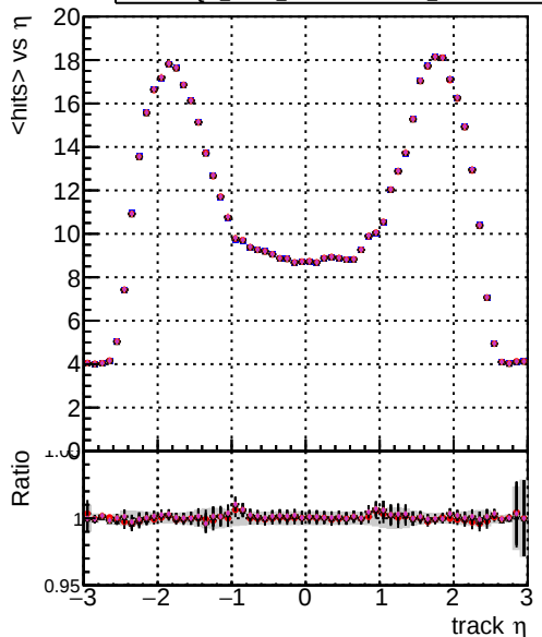
DOM mkFit TToriginal-106 DOM mkFit TTNEWHSMS95 ALLITERS-106 DOM mkFit TTNEWHSMS50 ALLITERS-106 DOM mkFit TTNEWHSMS100 ALLITERS-106
