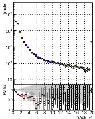
N of reco track vs. \chi^2 for BDM, mFit, TITAN, TITANsim, TITANsim+100, ALL, TITANsim+100+ALL
